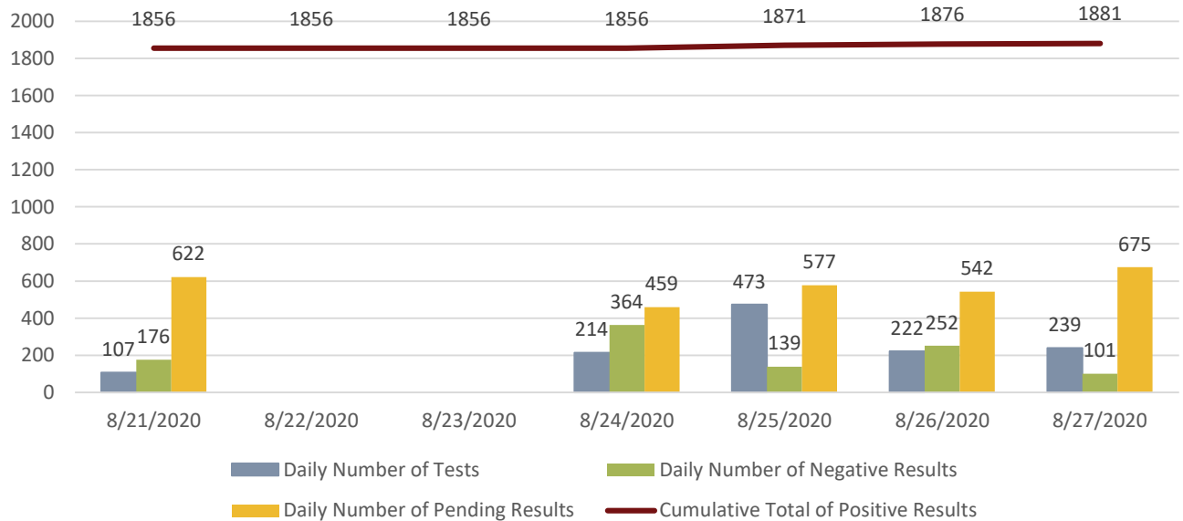
Number and Result of COVID-19 Tests Conducted at All USET Clinics
